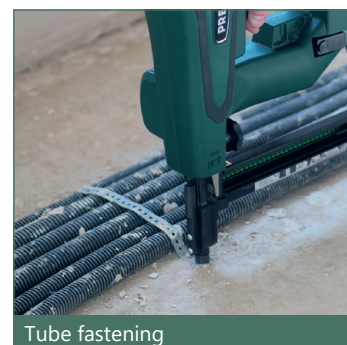
U-profile fastening
