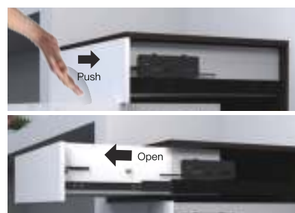
Push open and soft-close drawer adaptor 自彈抽屜裝置
