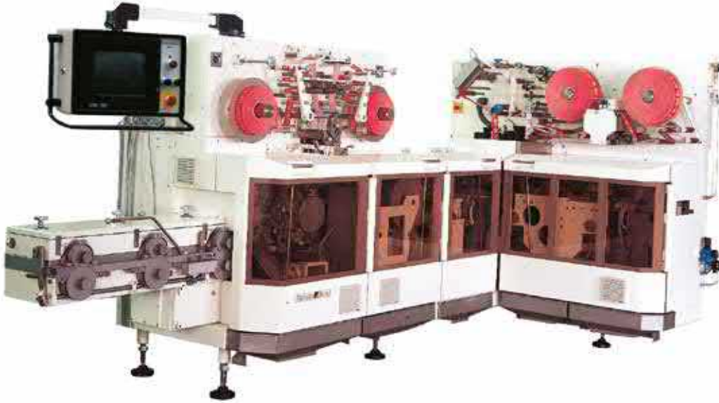
Stick Pack on edge Secondary packaging
